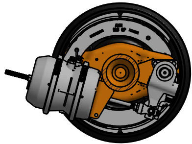
SECTION A-A SCALE 1/8
